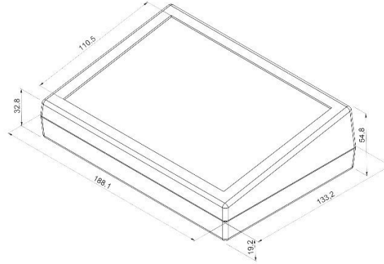
Figure 2: AT550-3 technical drawings
